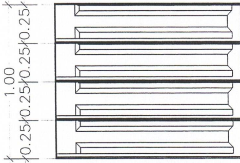
ELEVATION B SCALE 1:25
